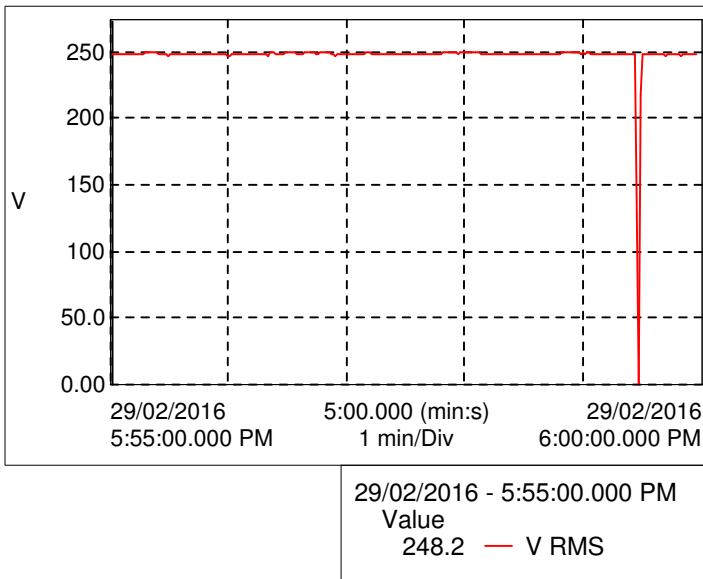
Graph - Voltage(Vrms)
