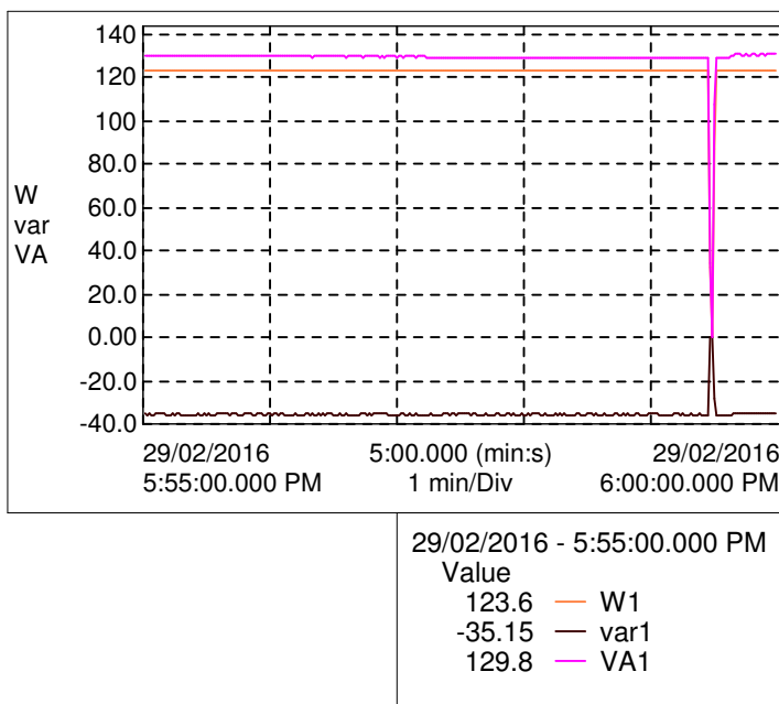
Graph - True Power(W)/Apparent Power(VA)/ Reactive Power(var)
