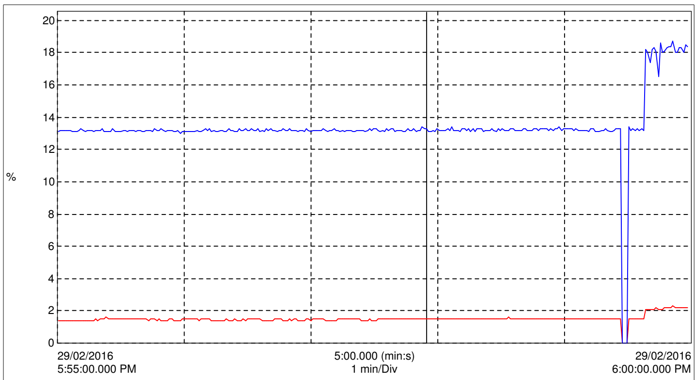
Graph - Total Harmonic Distortion - ATHD/VTHD
