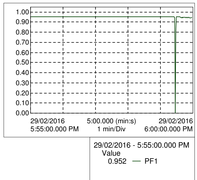
Graph - Power Factor ( PF)
