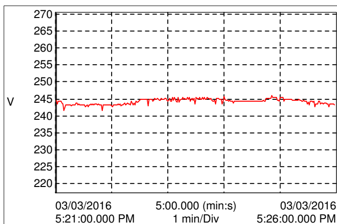
Graph - Voltage(Vrms)
