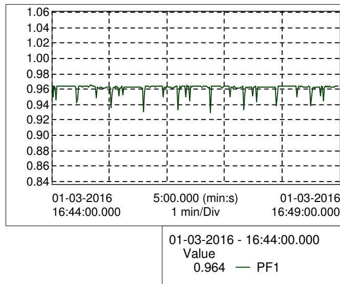
Graph - Power Factor (PF)
