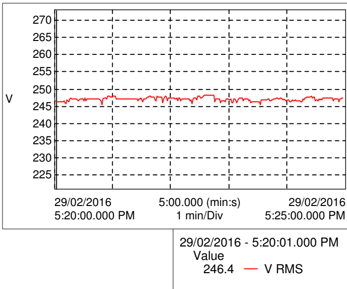
Graph - Voltage (Vrms)
