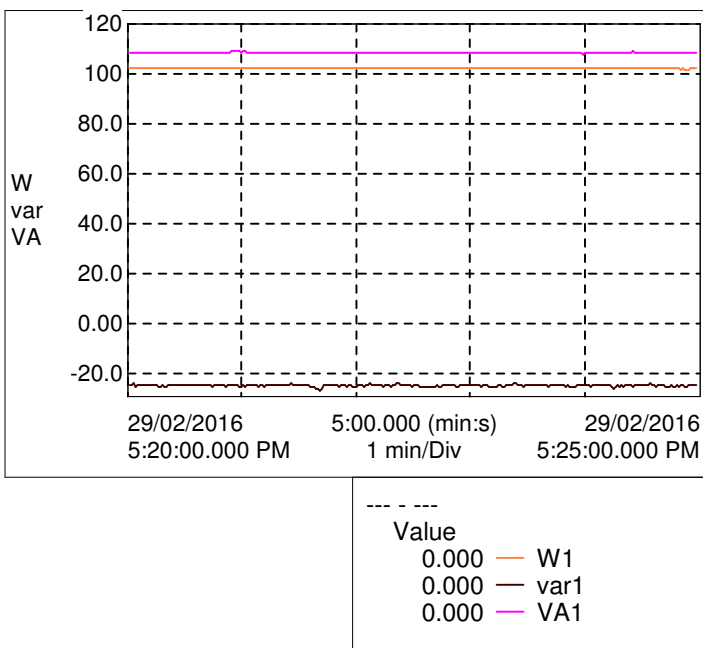
Graph - True Power(W)/Apparent Power(VA)/ Reactive Power(var)
