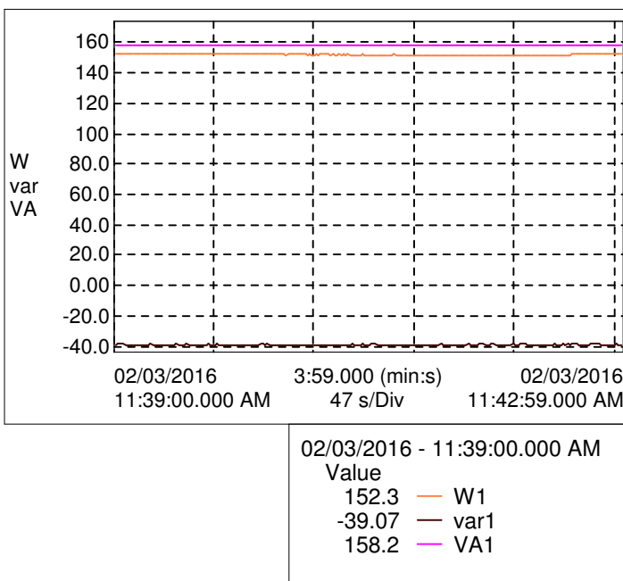
Graphs - True Power (W) / Apparent Power(VA)/ Reactive Power (var)
