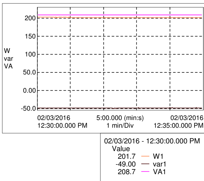
Graphs - True Power (W) / Apparent Power (VA) / Reactive Power (var)
