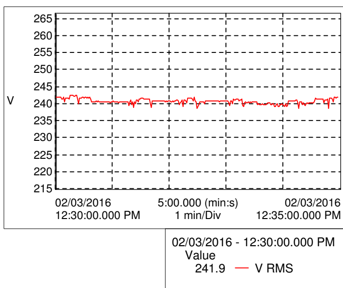
Graphs - Voltage (Vrms)
