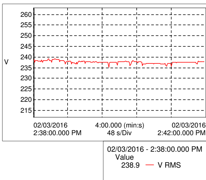
Graph - Voltage(Vrms)
