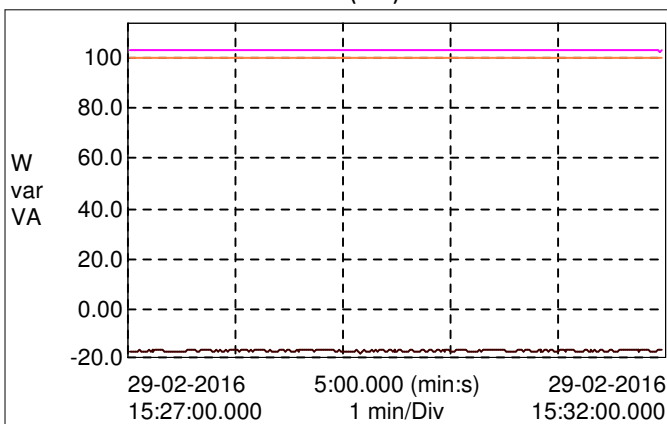
Graph - True Power(W)/Apparent Power(VA)/ Reactive Power(var)
