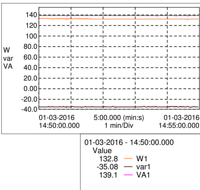
Graph - True Power(W)/Apparent Power(VA)/ Reactive Power(var)
