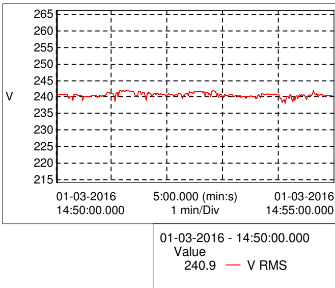
Graph - Voltage(Vrms)
