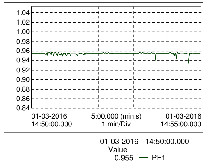
Graph - Power Factor(PF)
