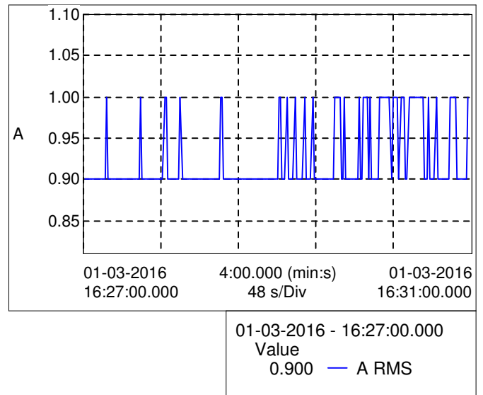
Graph - Current (Arms)
