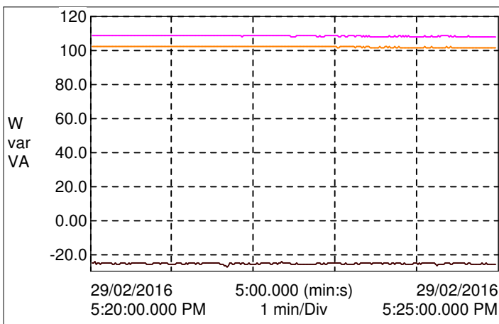
Graph - True Power(W)/Apparent Power(VA)/ Reactive Power(var)
