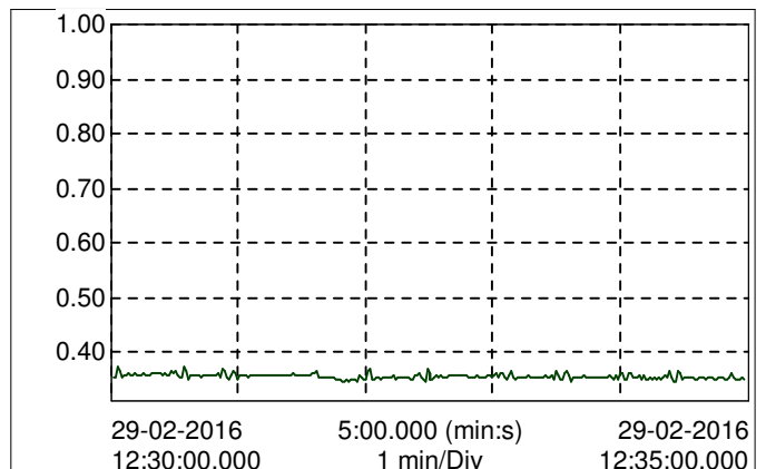
Graph - Power Factor (PF)
